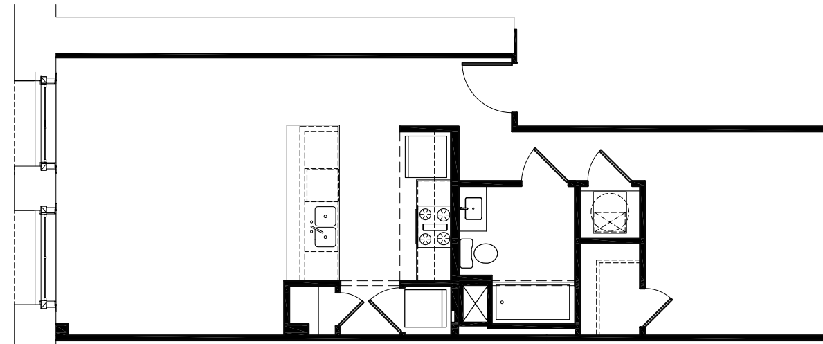
FLOOR PLAN - UNIT 202,302,402 and 502
